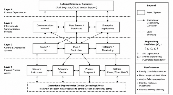
Figure 7. Operational Dependency Network Model.
